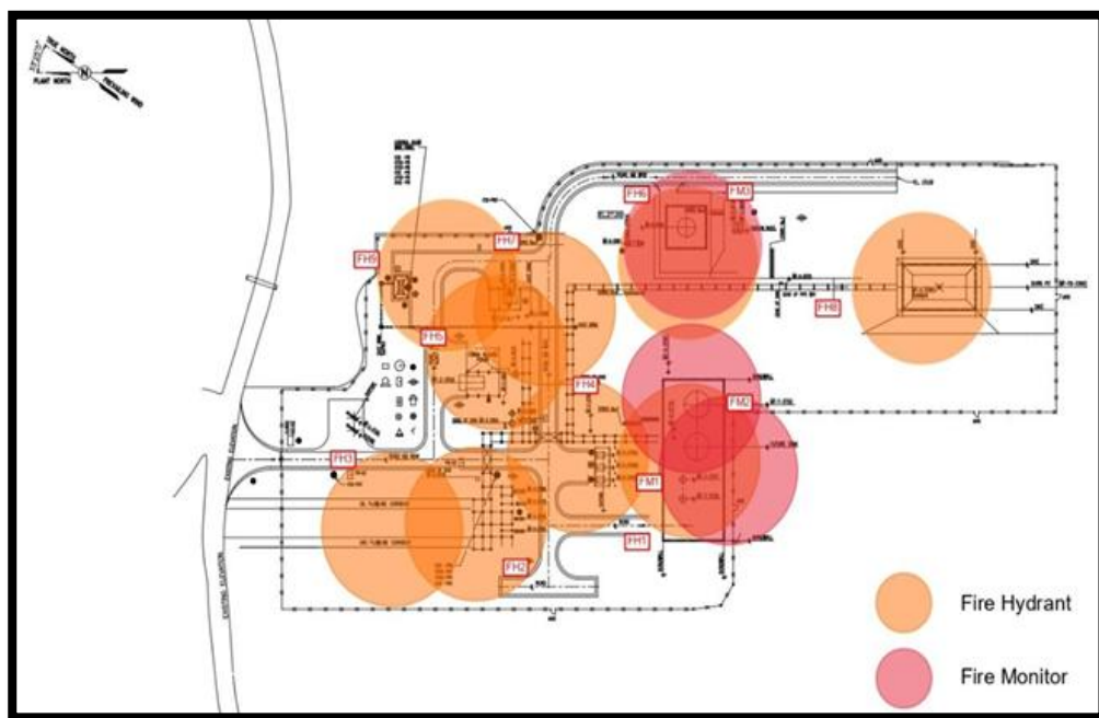
Figure 2. Mapping plan for fire hydrant & fire monitor at PT collection station
